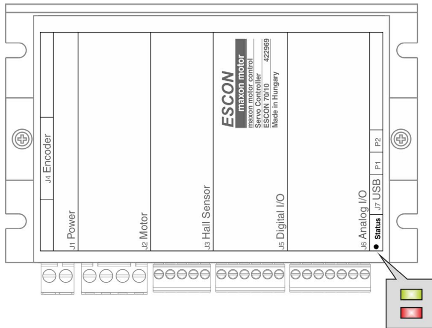
Figure 3-21 LEDs – Location
