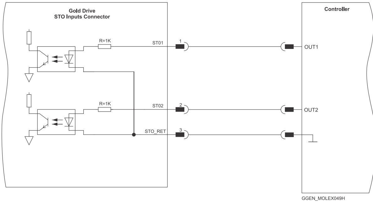
Figure 34: STO Input Connection – TTL Option
