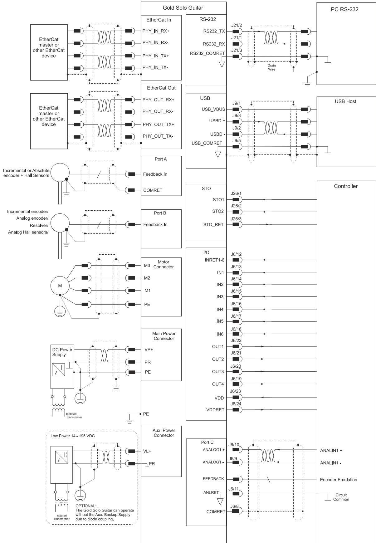
Figure 4: The Gold Solo Guitar Connection Diagram - EtherCAT
