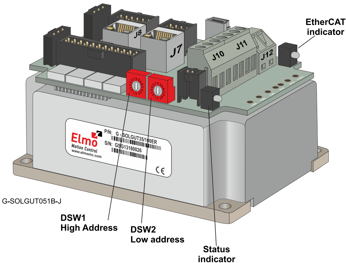
Figure 41: Position of EtherCAT Address Switches on the Gold Solo Guitar
