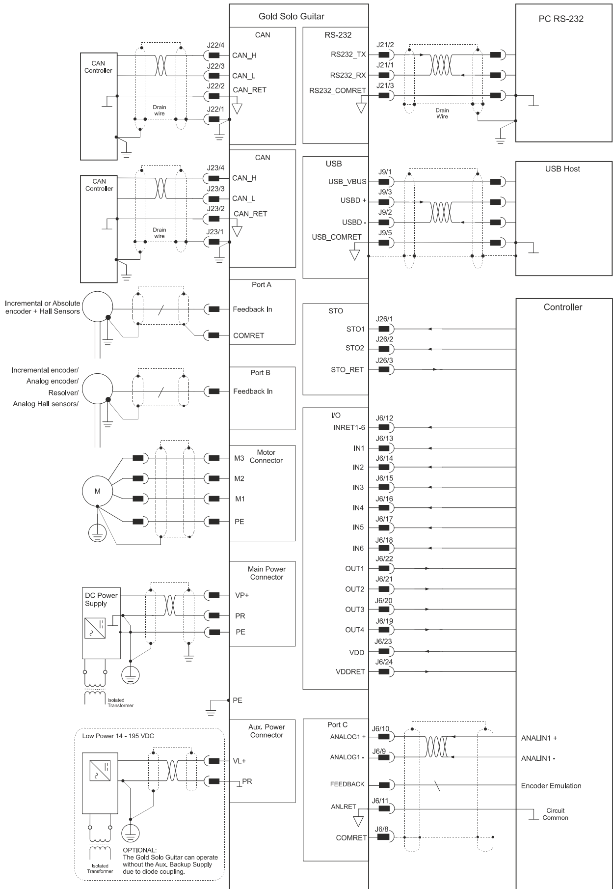
Figure 5: The Gold Solo Guitar Connection Diagram – CAN
