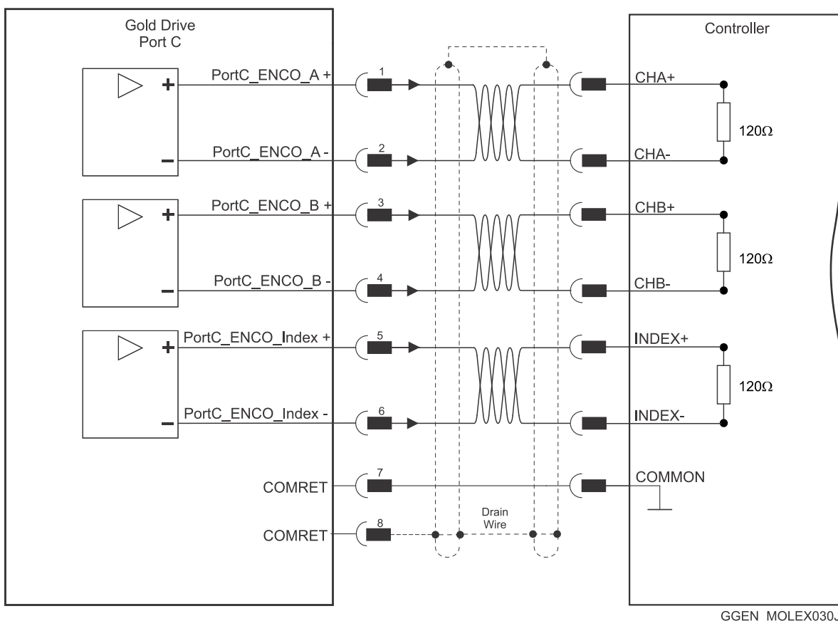
Figure 25: Encoder Differential Output – Recommended Connection Diagram
