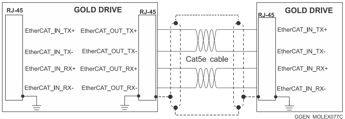
Figure 39: EtherCAT RJ-45 Connections
