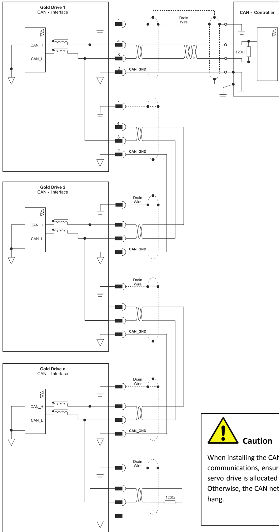
Figure 43: Gold Solo Guitar Connection Diagram – CAN
