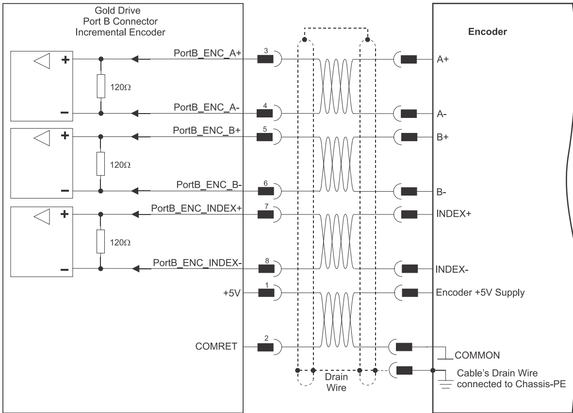
Figure 22: Port B Incremental Encoder Input – Recommended Connection Diagram
