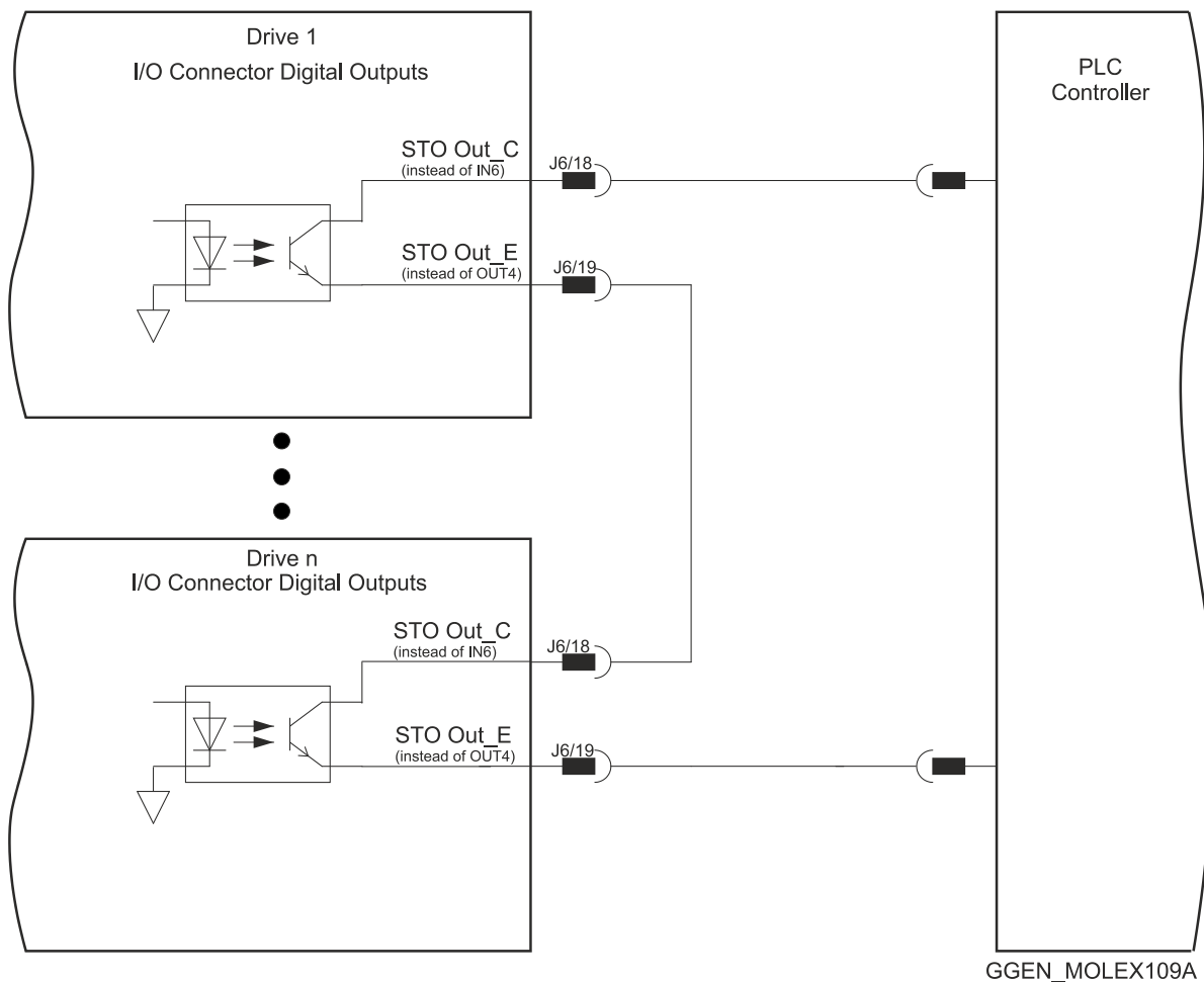
Figure 35: STO Output
