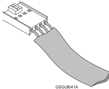
4-Pin Molex Plug
