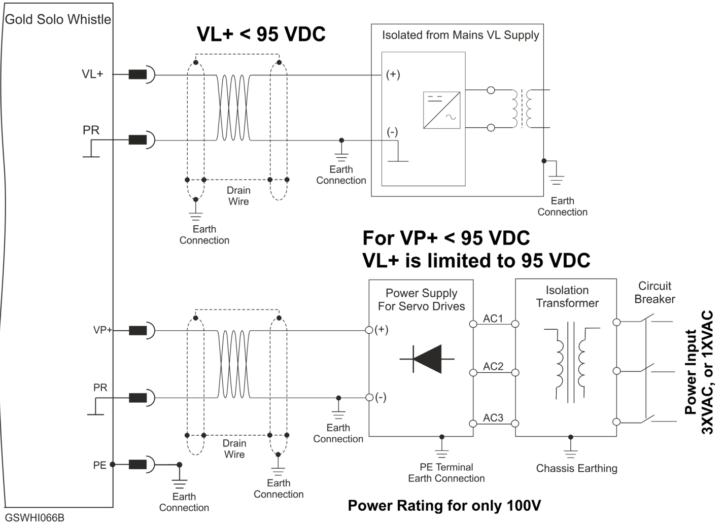
Figure 16: Auxiliary Supply Connection Diagram
