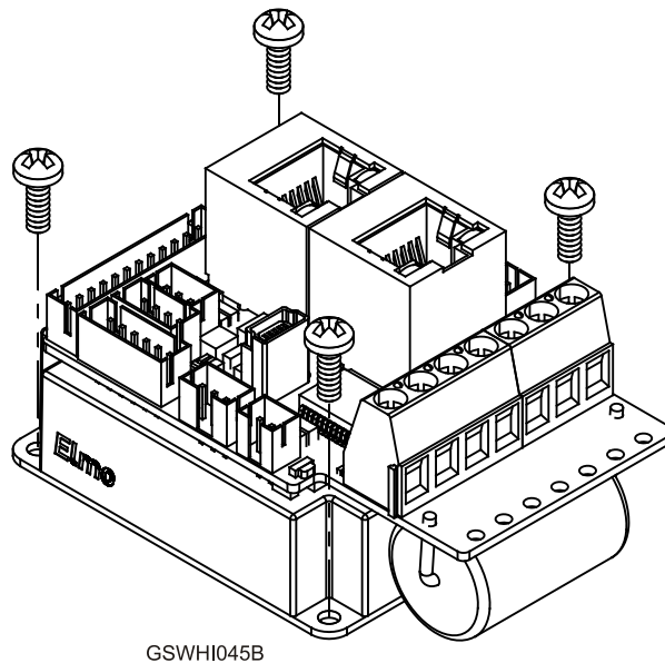
Figure 3: Mounting the Gold Solo Whistle
