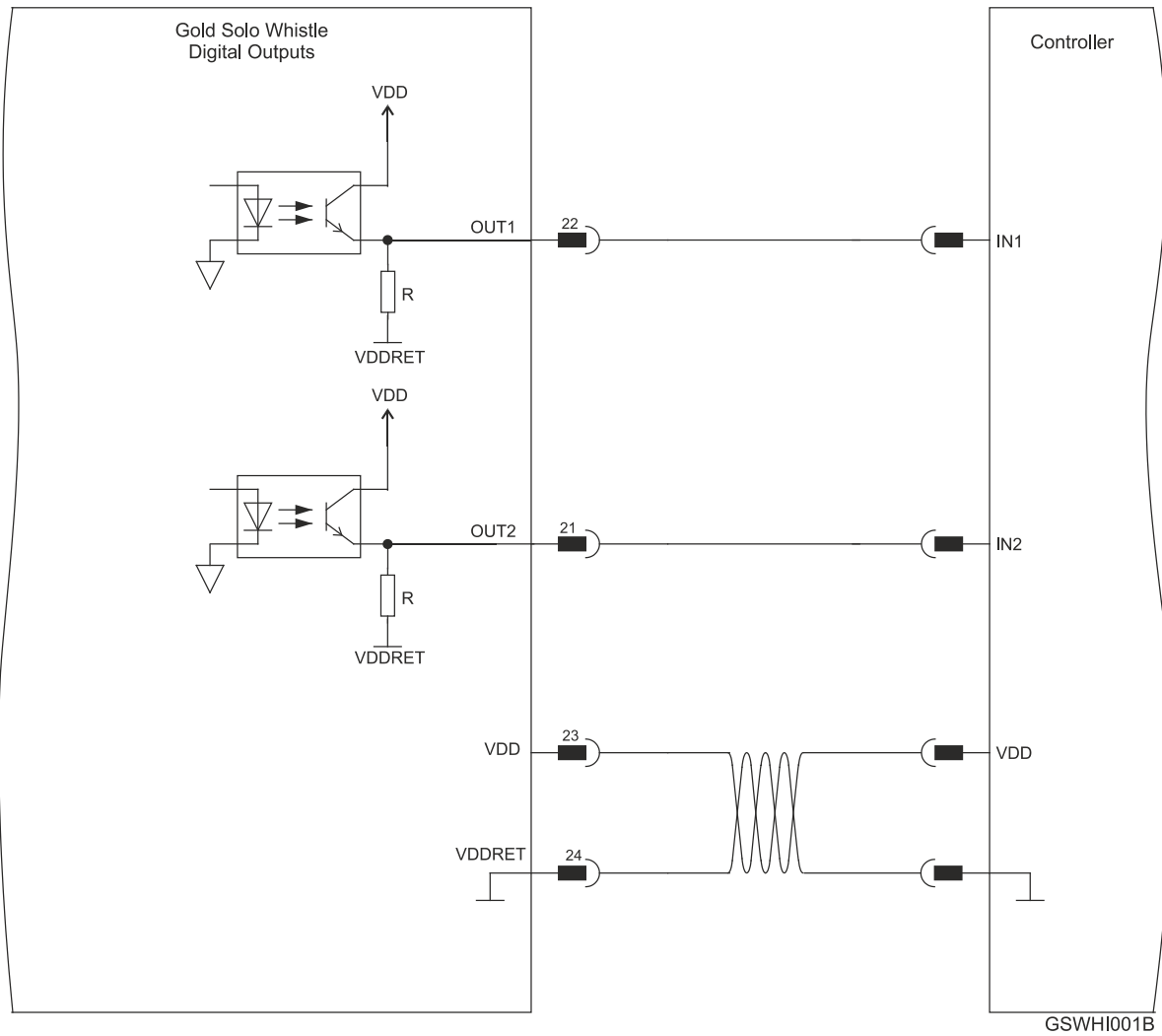
Figure 31: Digital Output Connection Diagram – TTL Option
