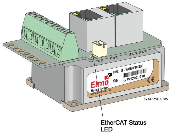
Figure 37: EtherCAT Status LED
