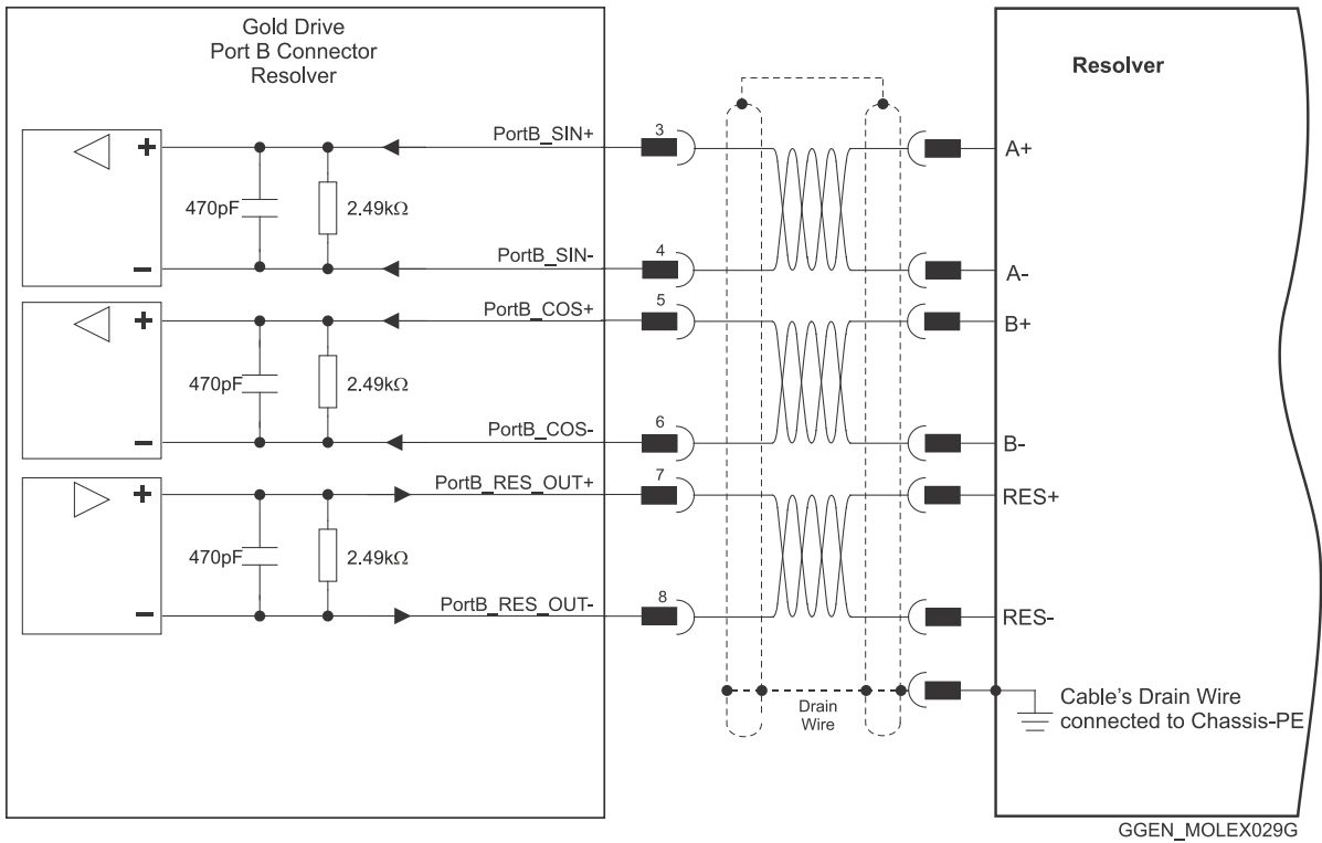
Figure 27: Port B – Resolver Shrouded Type Connection Diagram
