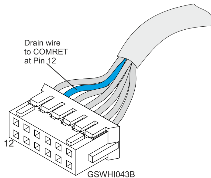
Figure 7: Feedback and Shrouded Control Cable Assemblies – Example
