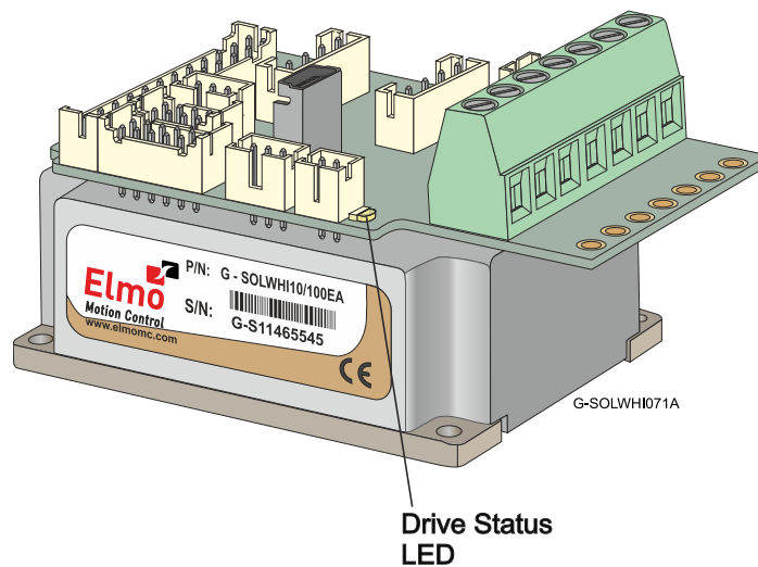
Figure 38: Gold Solo Whistle Status Indicator - CAN
