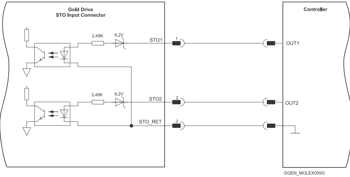
Figure 18: STO Shrouded Type Input Connection – PLC Source Option
