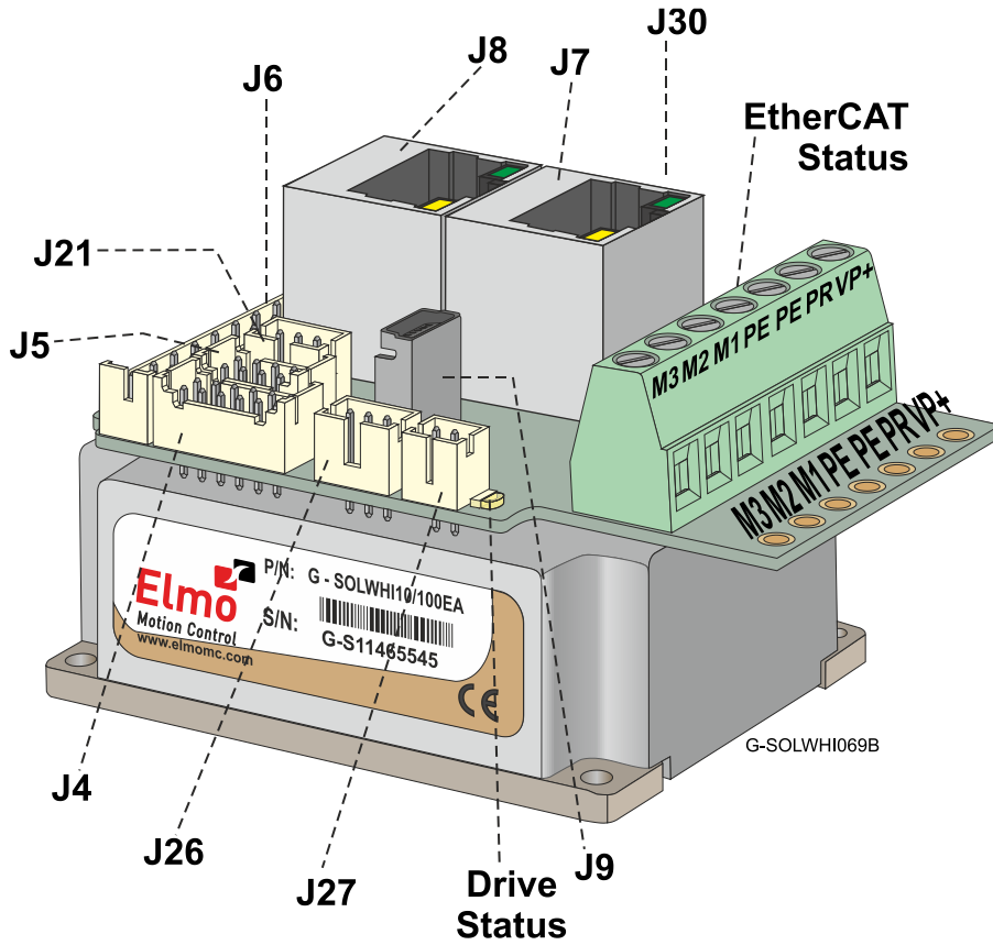
Figure 1: Connector Locations – EtherCAT
