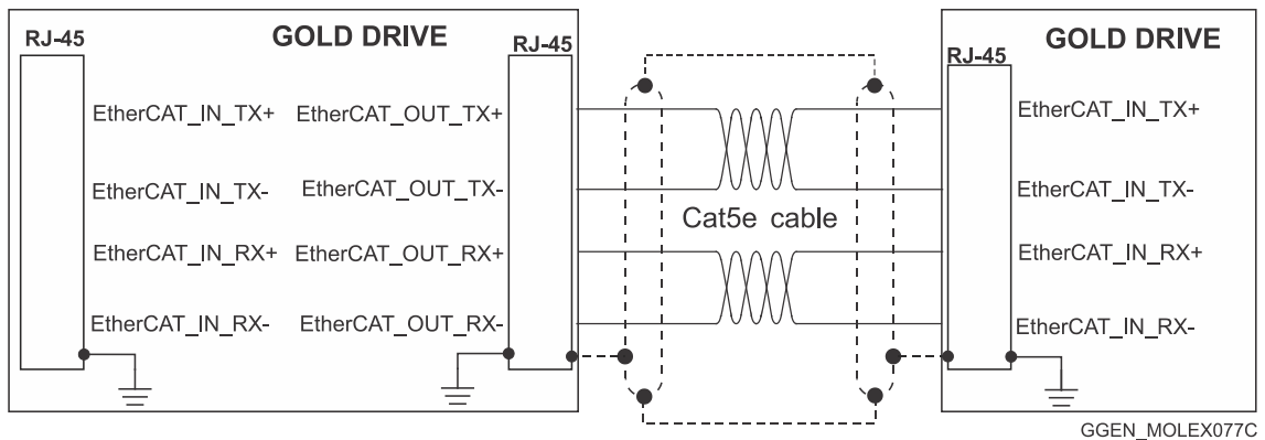
Figure 36: EtherCAT RJ-45 Connections
