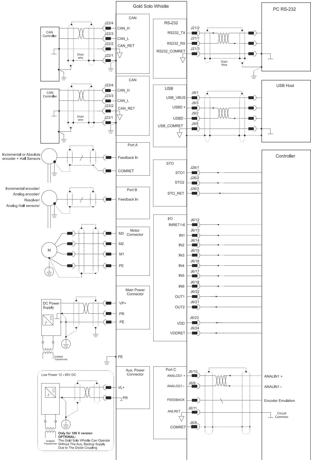
Figure 6: The Gold Solo Whistle Connection Diagram – CAN
