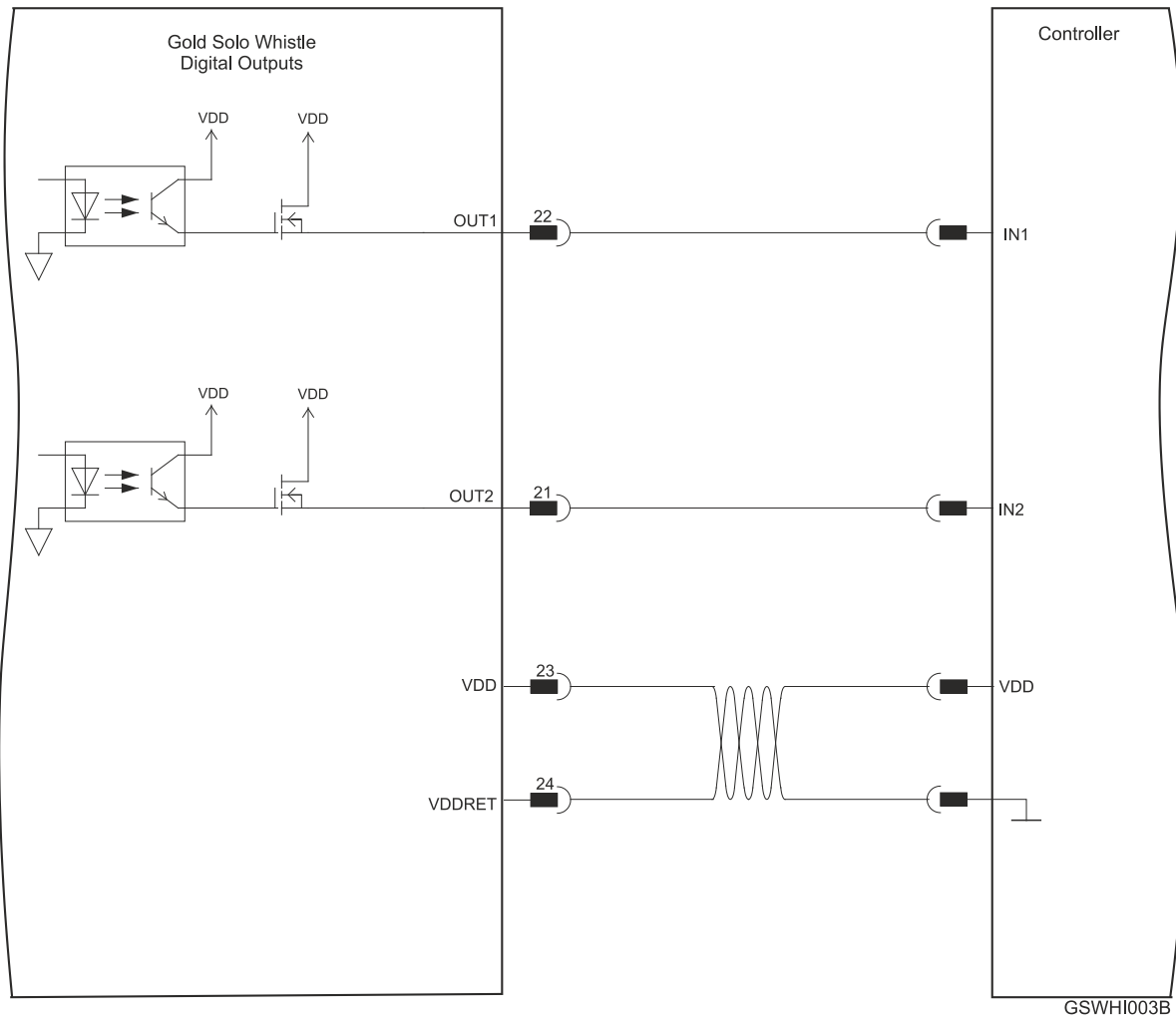
Figure 33: Digital Output Connection Diagram – Source PLC Option
