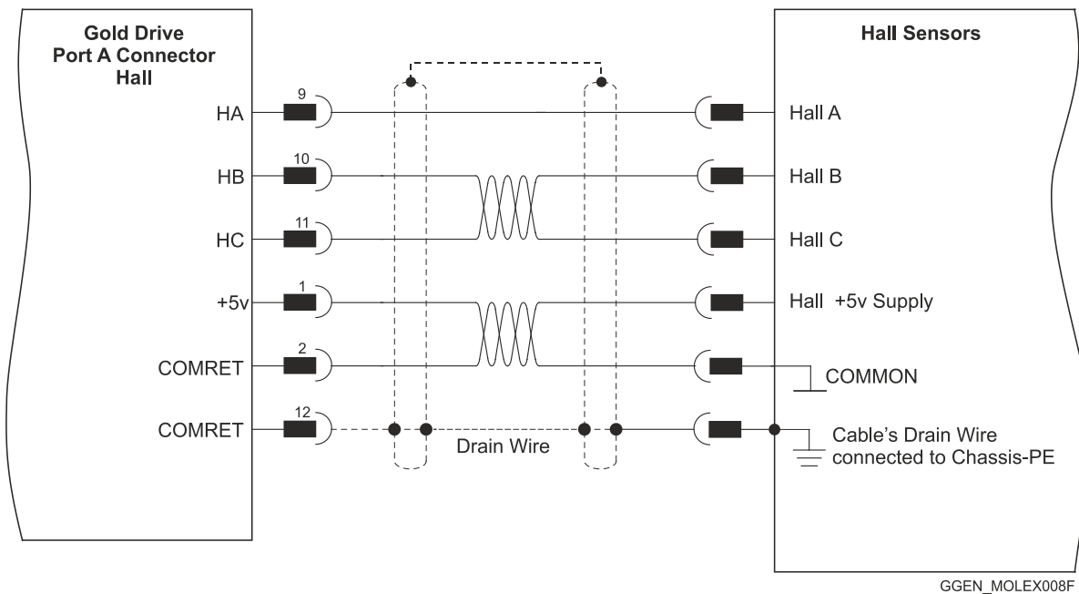
Figure 21: Shrouded Type Hall Sensors Connection Diagram
