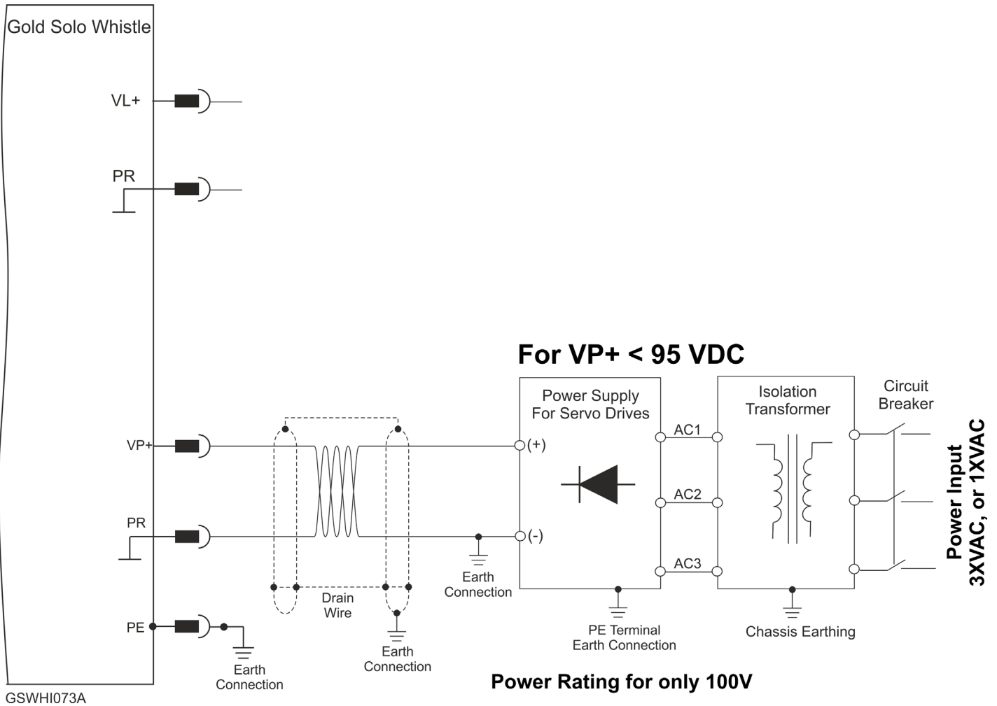
Figure 15: Main Power Supply Connection Diagram (No Auxiliary Supply)
