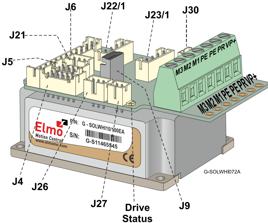
Figure 2: Connector Locations – CAN
