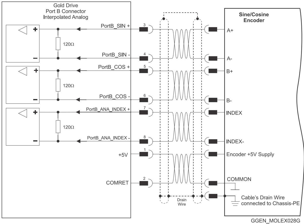
Figure 26: Port B - Interpolated Analog Encoder Shrouded Type Connection Diagram
