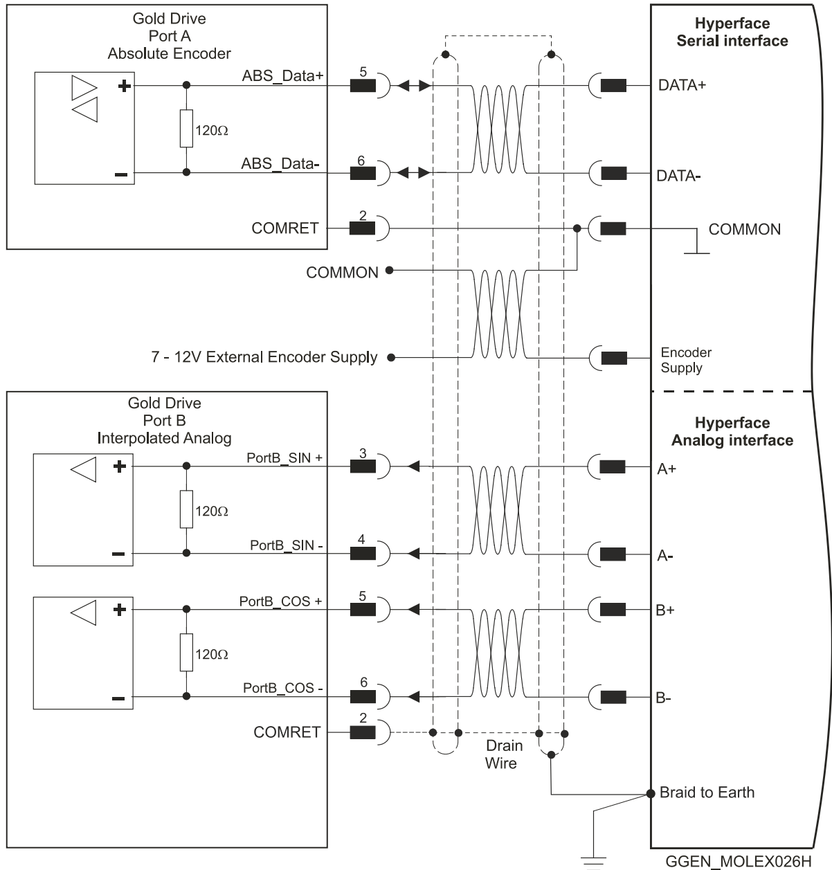
Figure 24: Absolute Serial Encoder – Recommended Shrouded Type Connection Diagram for Stegmann Hiperface
