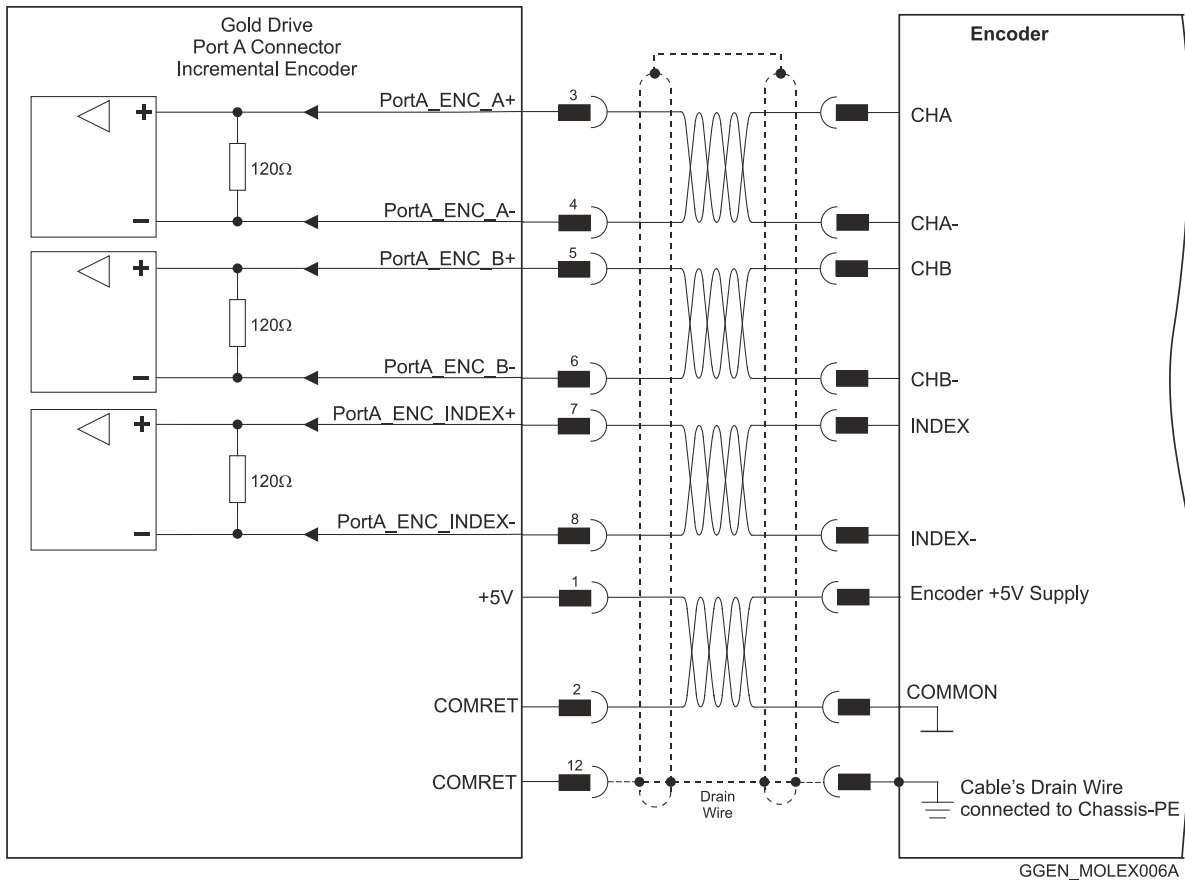
Figure 20: Port A Shrouded Type Incremental Encoder Input – Recommended Connection Diagram
