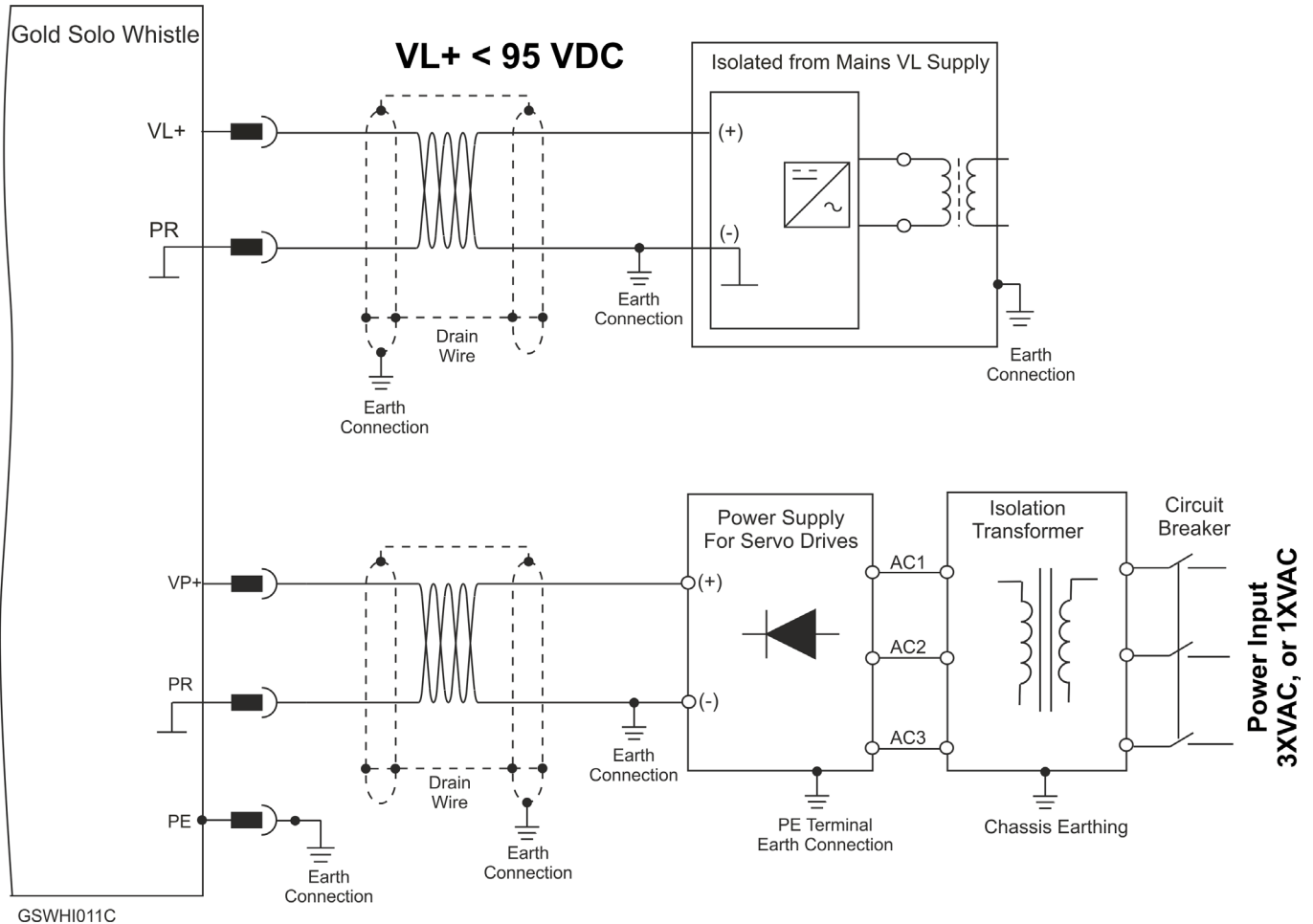
Figure 14: 200 VDC Power Source Connection Diagram
