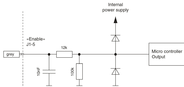
Figure 17 5-Wire Variant: Internal Circuitry of Input “Enable”
