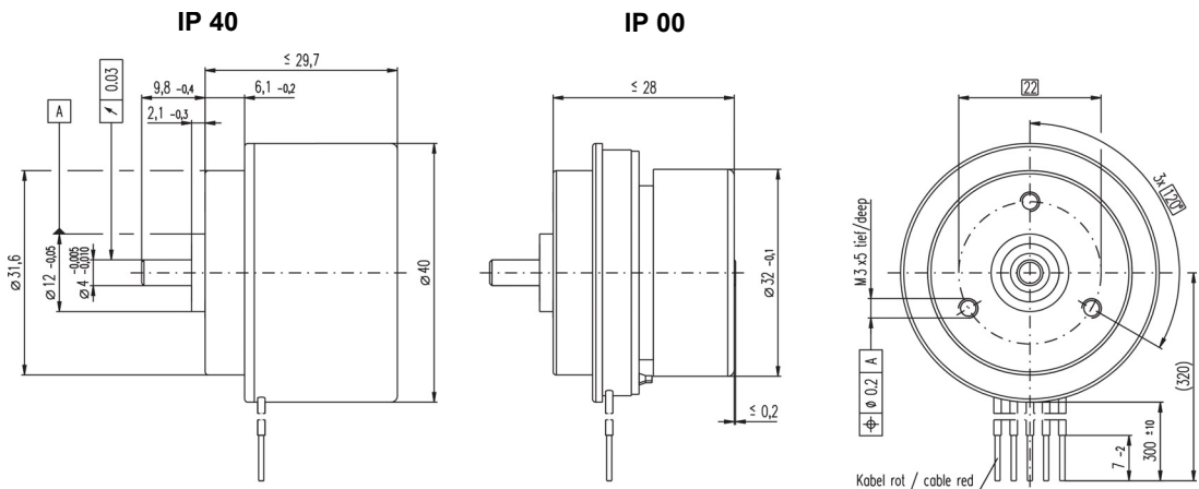
Figure 4 15 Watt Version – Dimensional Drawing [mm]
